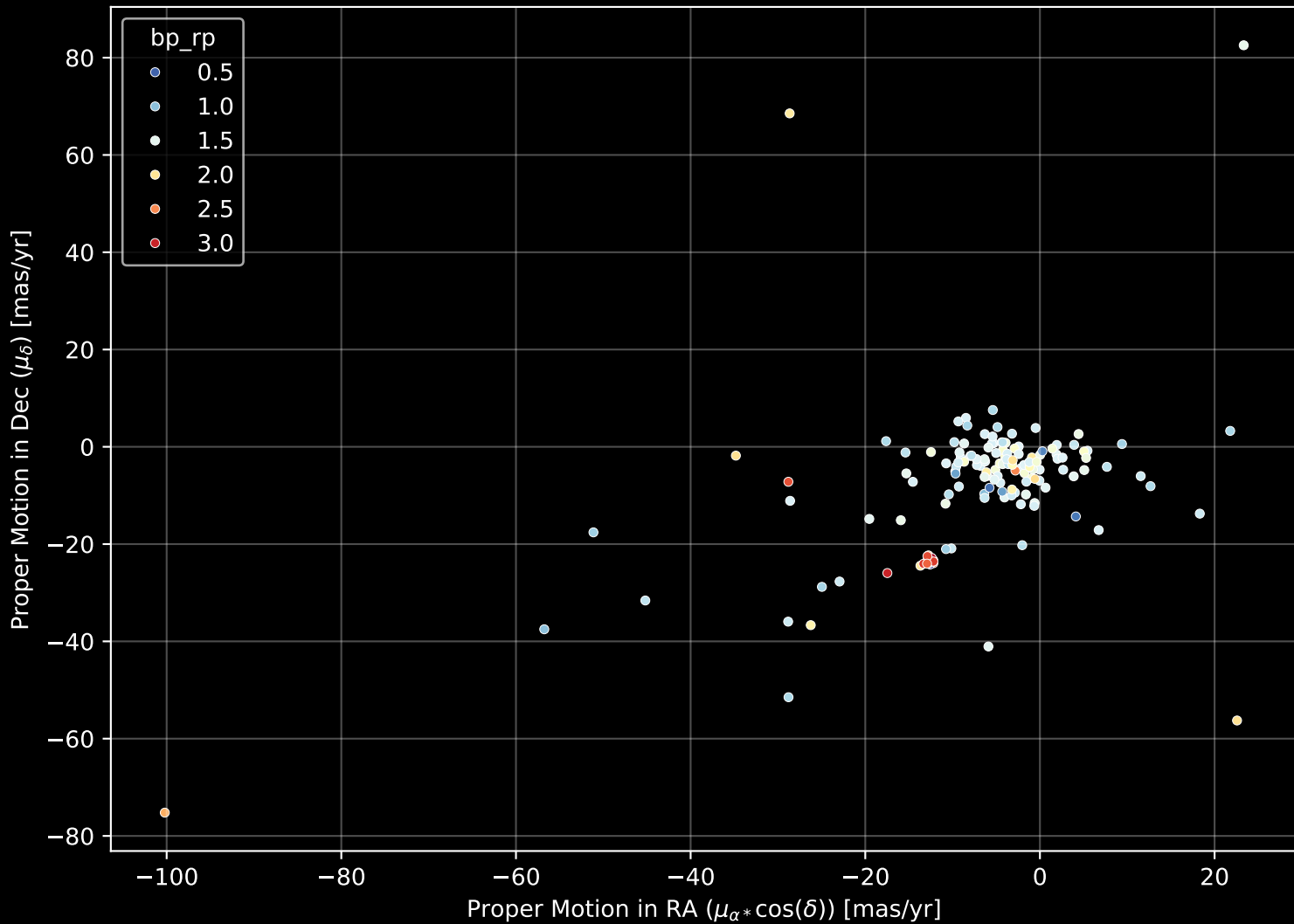
APOGEE DR17 Field: [K2_C2_350+23] Proper Motion Diagram (n= 148)
