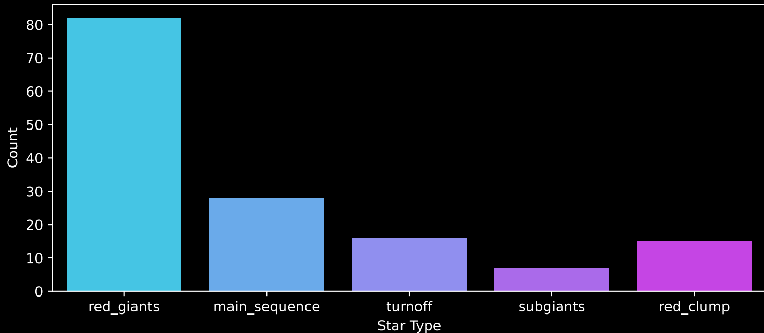
APOGEE DR17 Field: [K2_C2_350+23] Count plot of Star Type
