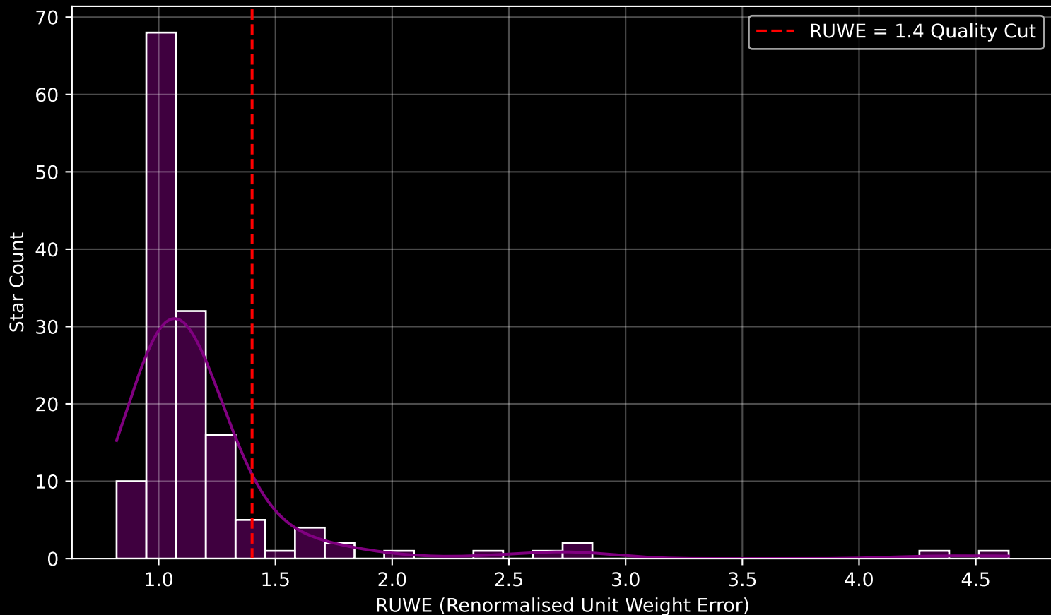
GAPOGEE DR17 Field [K2_C2_350+23] RUWE Distribution (n= 145)
