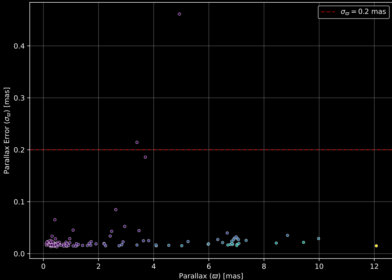
APOGEE DR17 Field: [K2_C2_350+23] Parallax Quality (n= 148)
