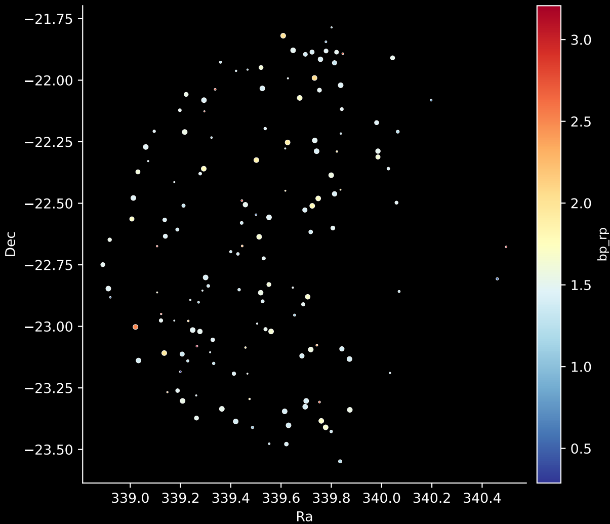
APOGEE DR17 Field: [K2_C2_350+23] Stars: 148
