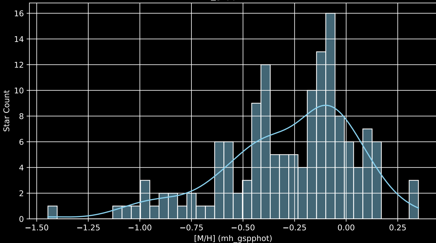
APOGEE DR17 Field: [K2_C2_350+23 [M/H] (mh_gspphot) (n= 147)
